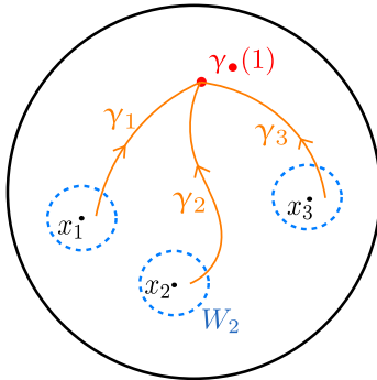
Figure 1. A positively 3-pathed Riemann sphere with local coordinates
