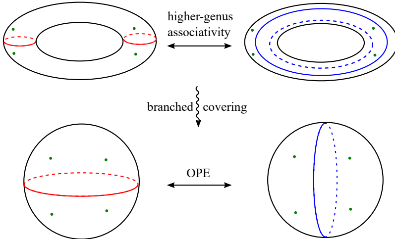
Figure 2. The permutation-twisted OPE is equivalent to an associativity of (possibly) higher genus conformal blocks via the permutation covering.
