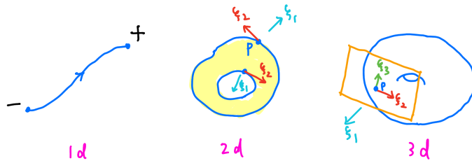
Figure 35.1. Boundary orientations
